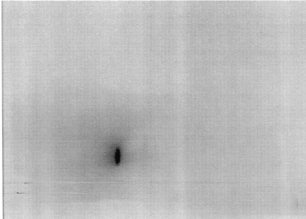
Figure 5 - Image of the monochromator's slit on the CCD EEV-02-06 at \lambda = 1321 Å. The dimensions of the CCD are 578 \times 385 pixels with a pixels size of 22 \mu\text{m}^2 .
